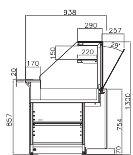
VKBNA - VD neutra aberta neutral opened neutre ouverte neutra abierta
