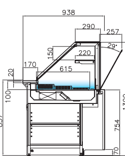
VKBCHS - VD 3S chocolates chocolate chocolat chocolate
